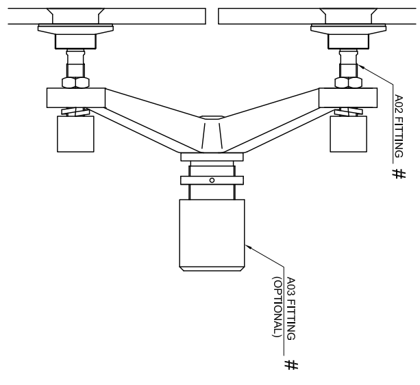
REAR VIEW ON FITTING (SCALE 1:4 (A4))
